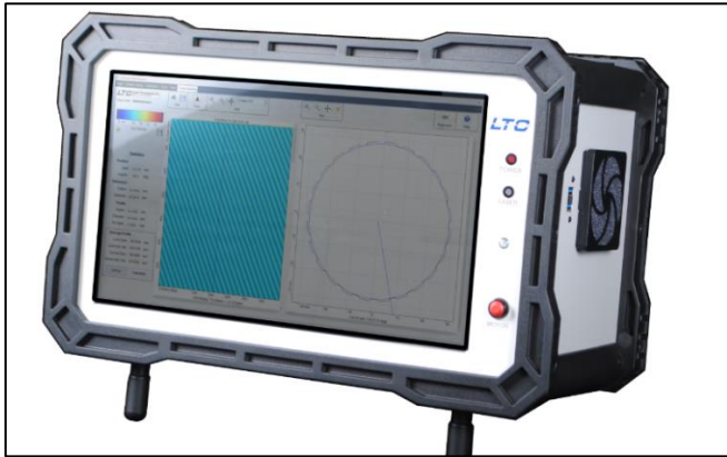
LP-5000™ Front View
